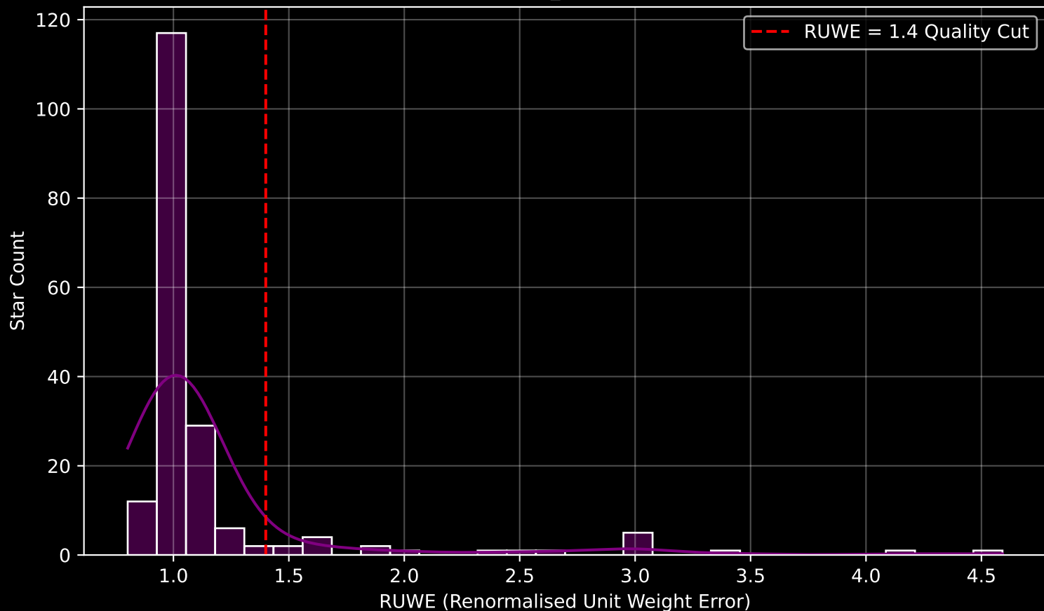
GAPOGEE DR17 Field [099+56_btx] RUWE Distribution (n= 186)
