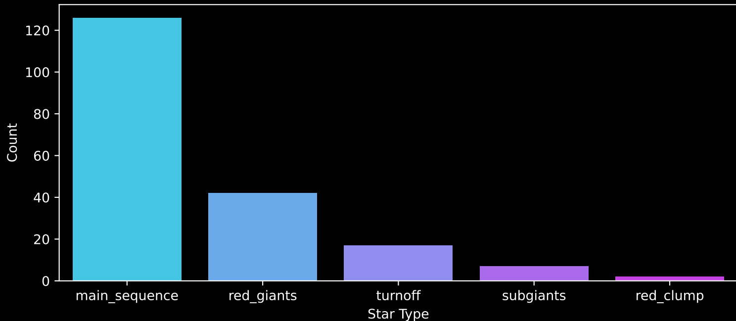
APOGEE DR17 Field: [099+56_btx] Count plot of Star Type
