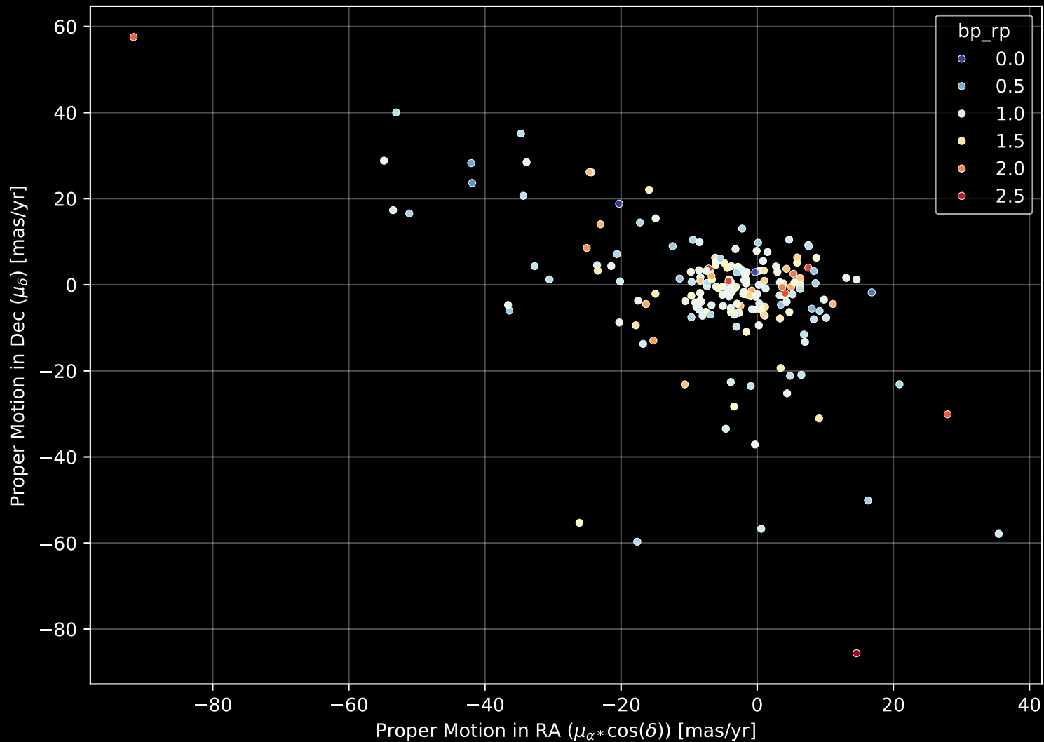
APOGEE DR17 Field: [099+56_btx] Proper Motion Diagram (n= 194)
