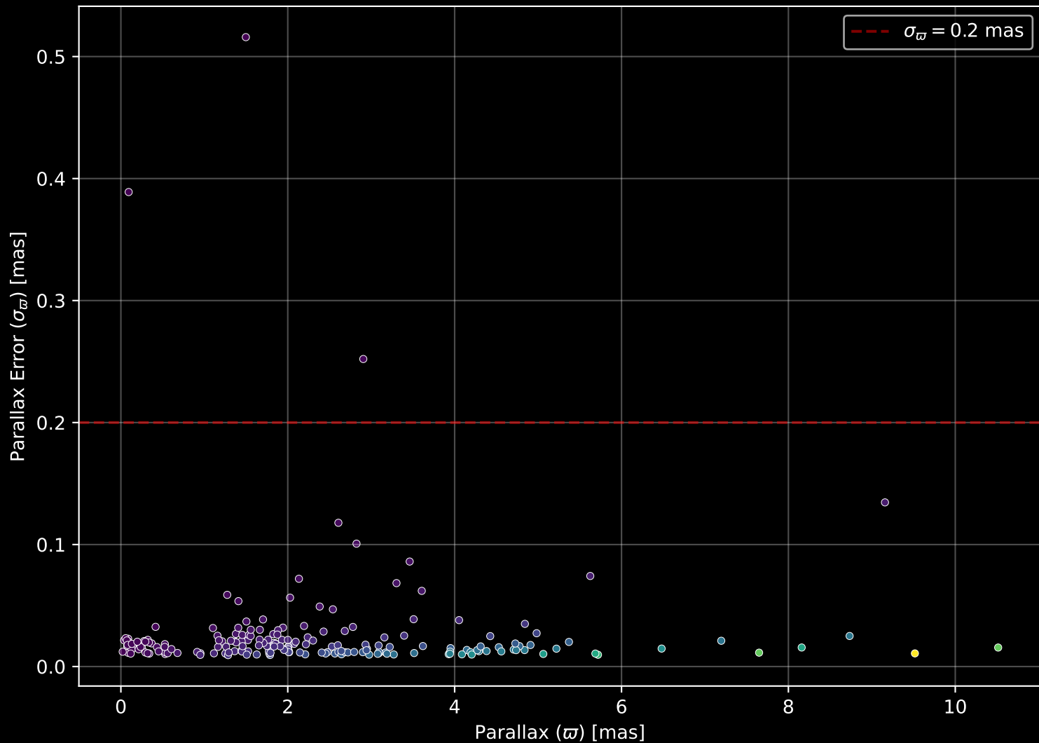
APOGEE DR17 Field: [099+56_btx] Parallax Quality (n= 194)
