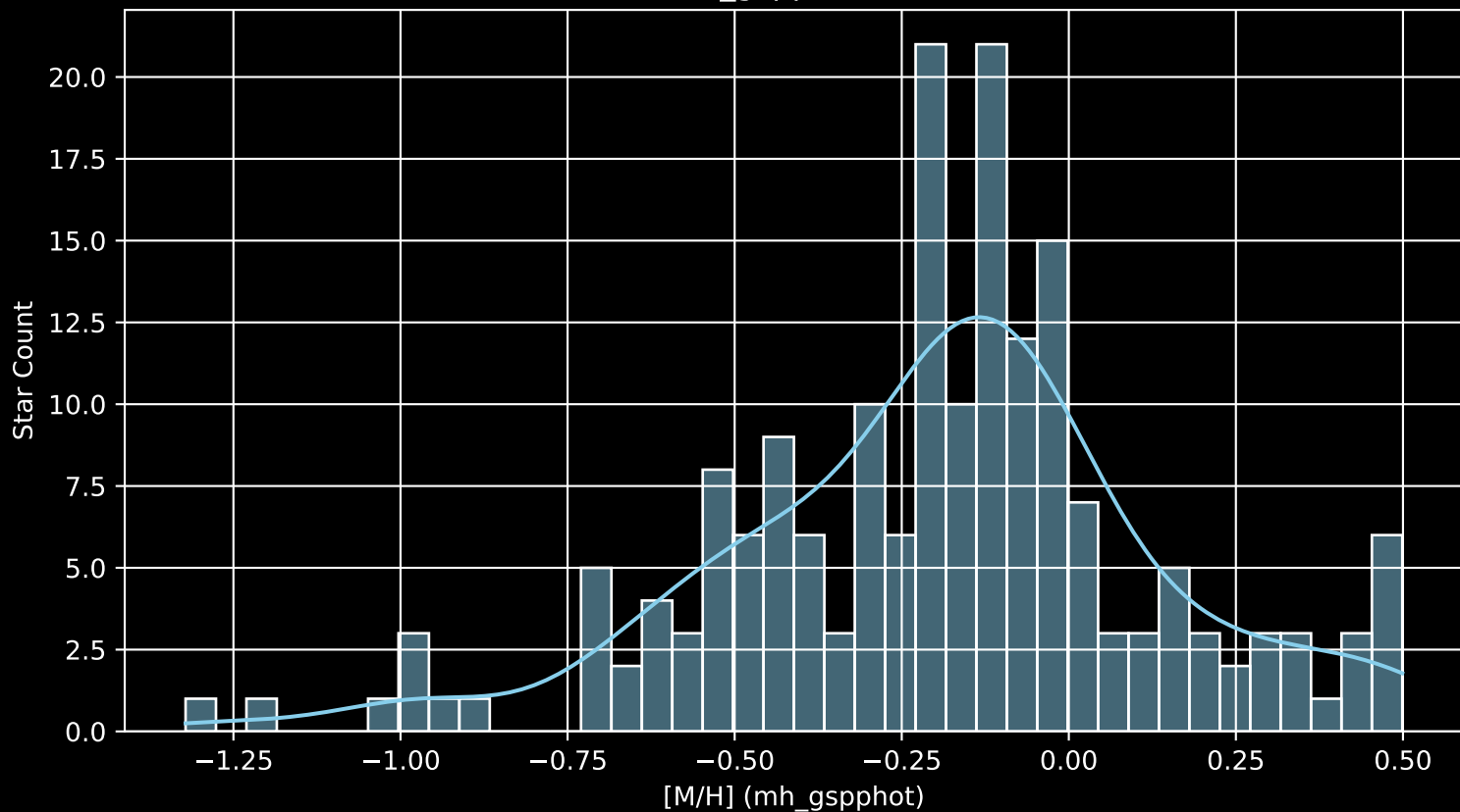
APOGEE DR17 Field: [099+56_btx [M/H] (mh_gspphot) (n= 188)
