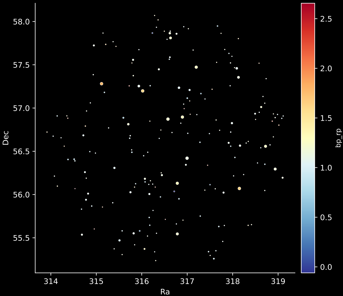
APOGEE DR17 Field: [099+56_btx] Stars: 194
